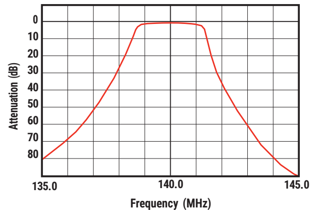
TYPICAL RESPONSE CURVES
