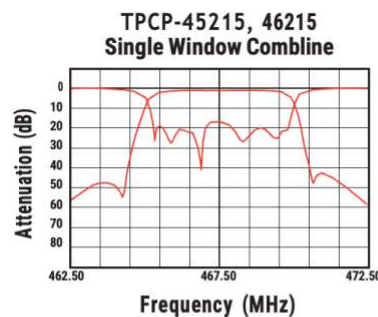
TYPICAL FILTER RESPONSE CURVES
