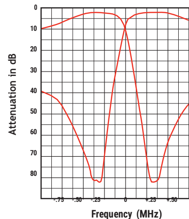
TYPICAL RESPONSE CURVES (TPRD-1484)
