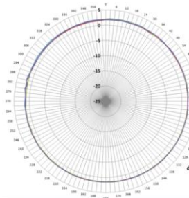
Horizontal Beam Pattern
