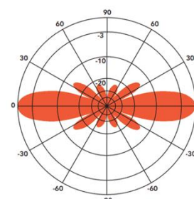
Vertical Beam Pattern
