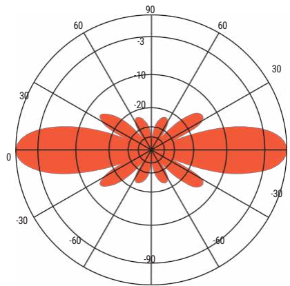
ANT500F6 - 490 MHz Vertical Plane Gain = 6.28 dBd
